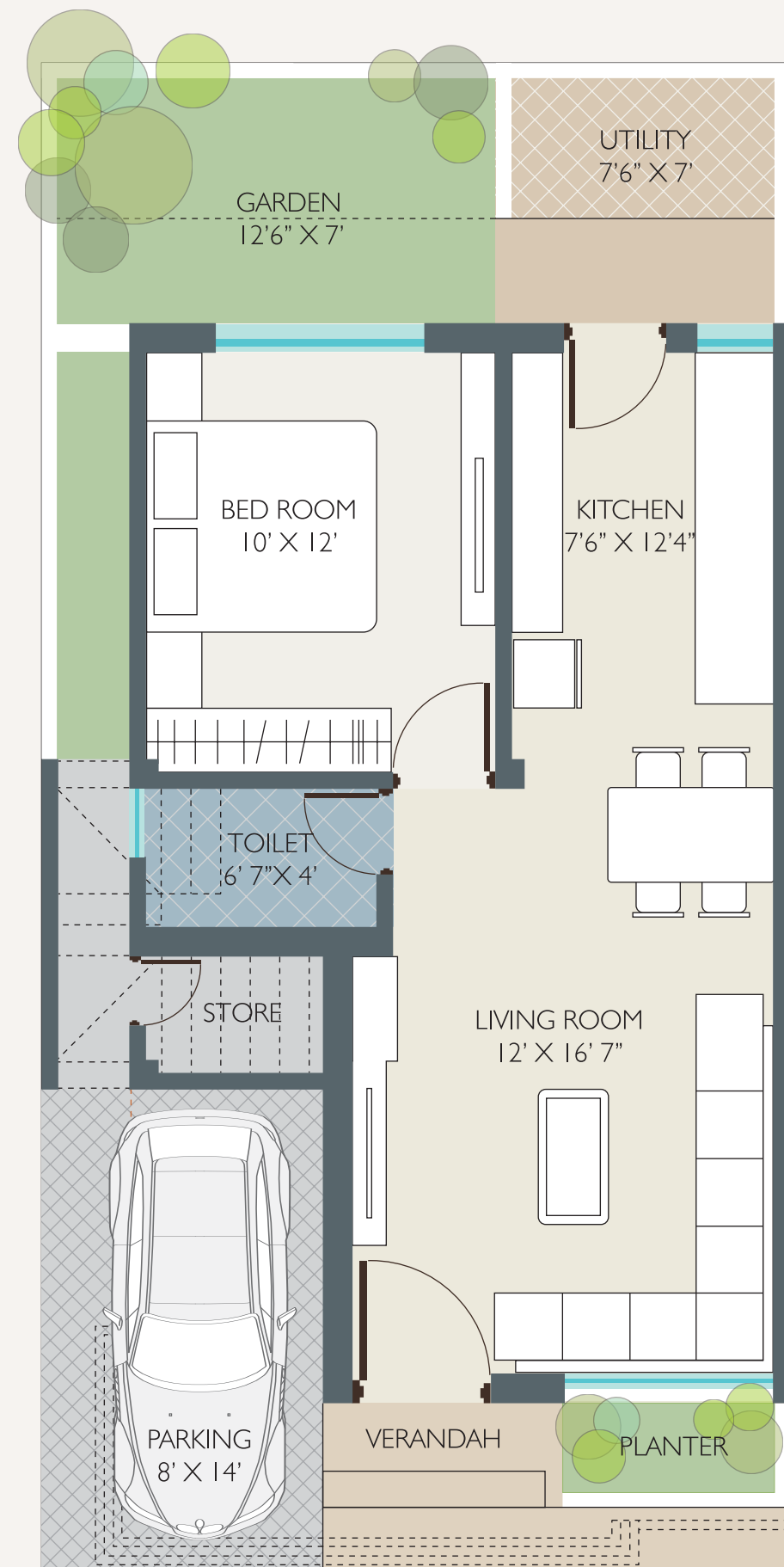
GROUND FLOOR
